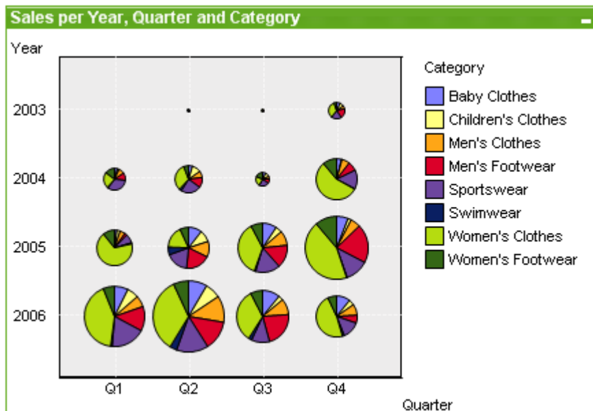
Grid chart
