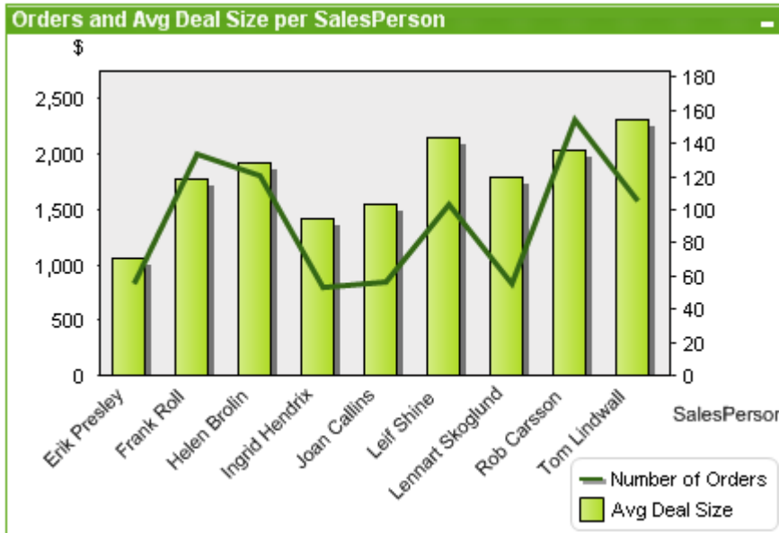
Combo chart
