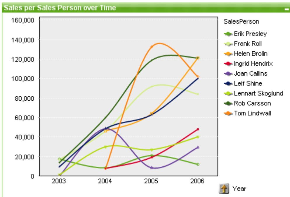
Line chart
