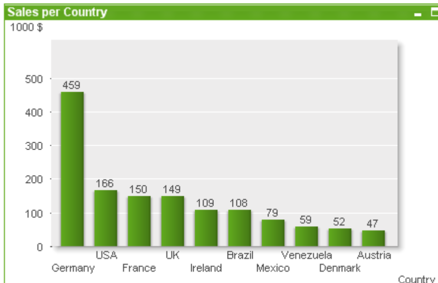
Bar Chart
