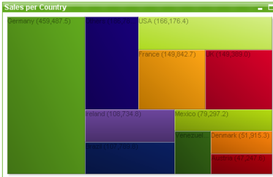
Block chart
