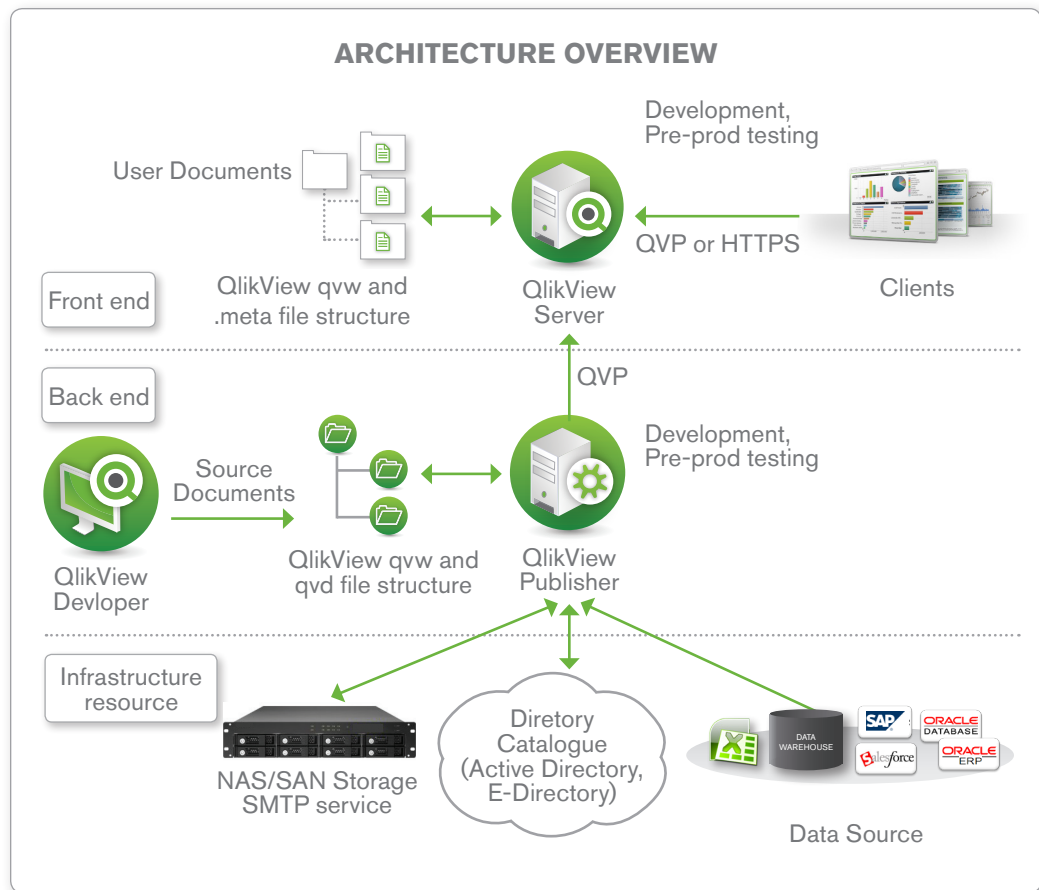
Figure 1: Architecture Overview
