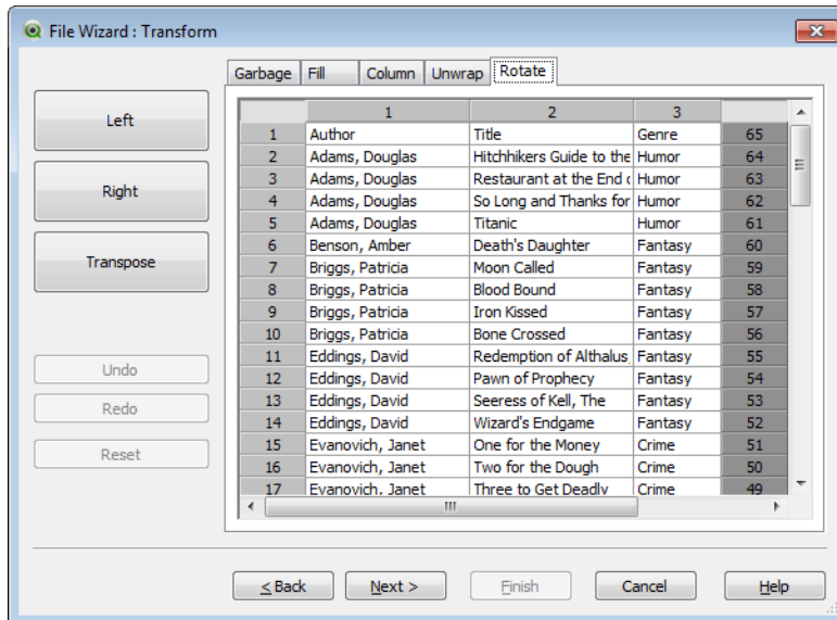
File Wizard: Transform, Rotate tab
