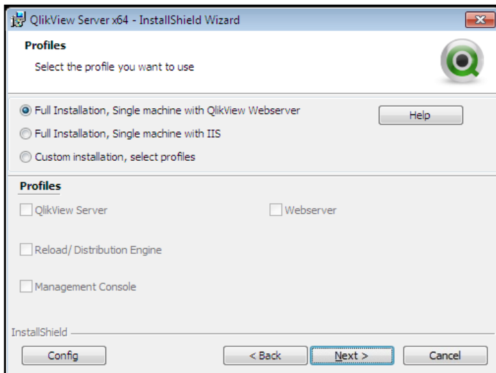
Profiles dialog
